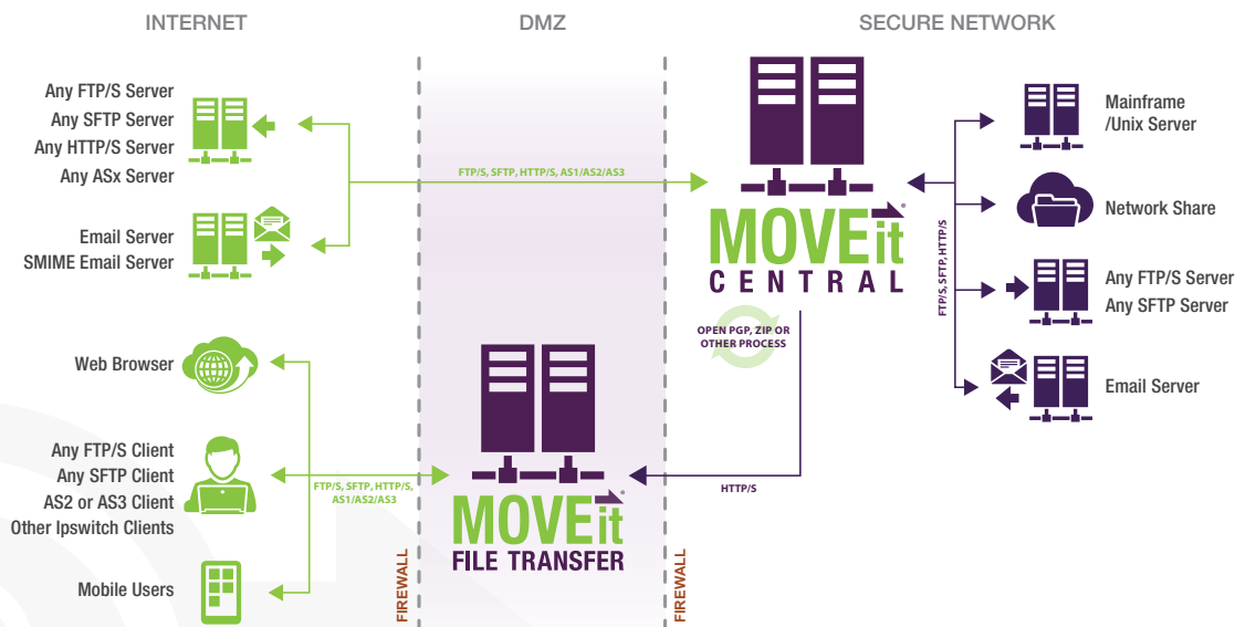
MOVEit Central Architecture
